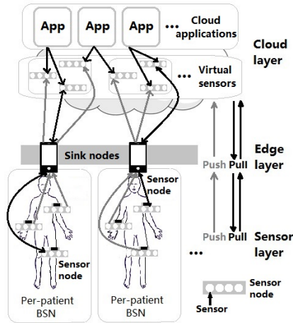
Figure 1: A Push-Pull Hybrid Communication in BitC
