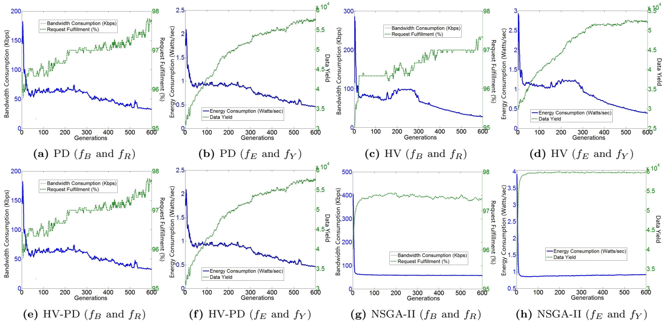
Figure 2: Objectives Values through Generations with BitC Variants and NSGA-II
